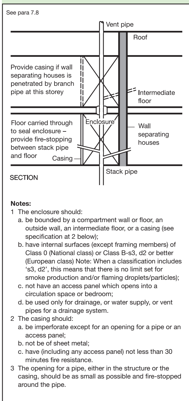
Diagram 15 Enclosure for drainage or water supply pipes
