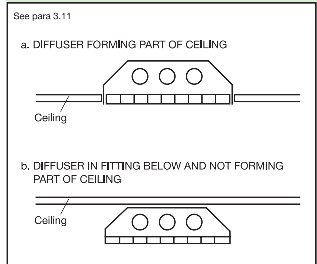
Diagram 8 Lighting diffuser in relation to ceiling
