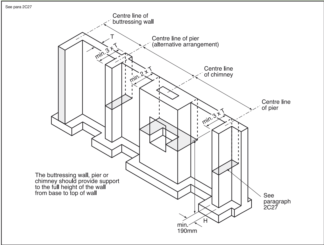
Diagram 13 Buttrressing
