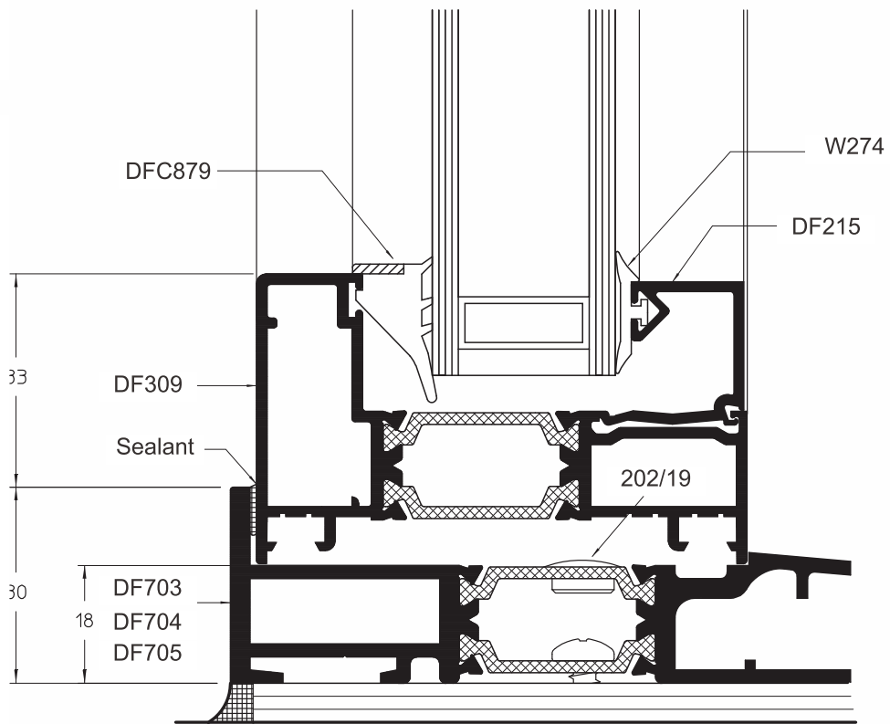
SUBCILL/FIXED LIGHT/SQUARE BEAD
