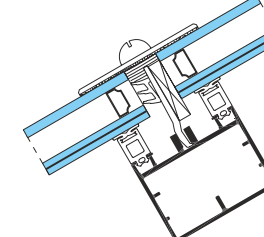
MX Sloped with Trame Verticale
