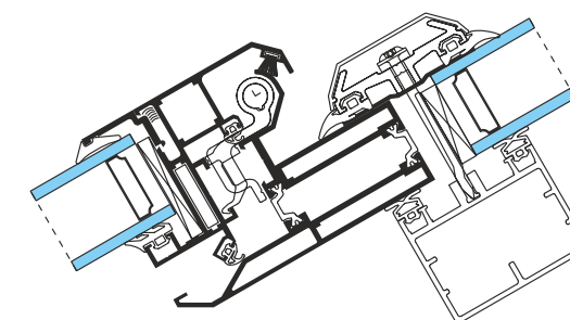
MX Roof-mounted opening vent
