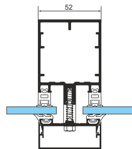
MX single glazing Visible grid
