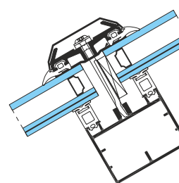
MX Sloped, Visible Grid
