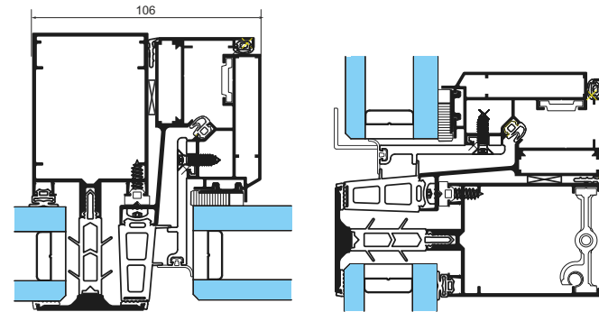
Top-hung open-out vent
