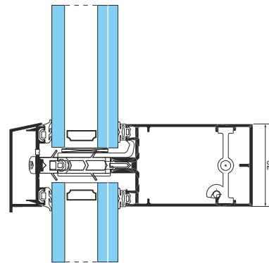
Vertical section Visible grid or Trame Horizontale
