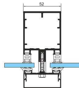
MX SG single glazing Trame Verticale
