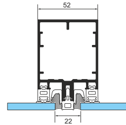
MX single glazing Trame Horizontale
