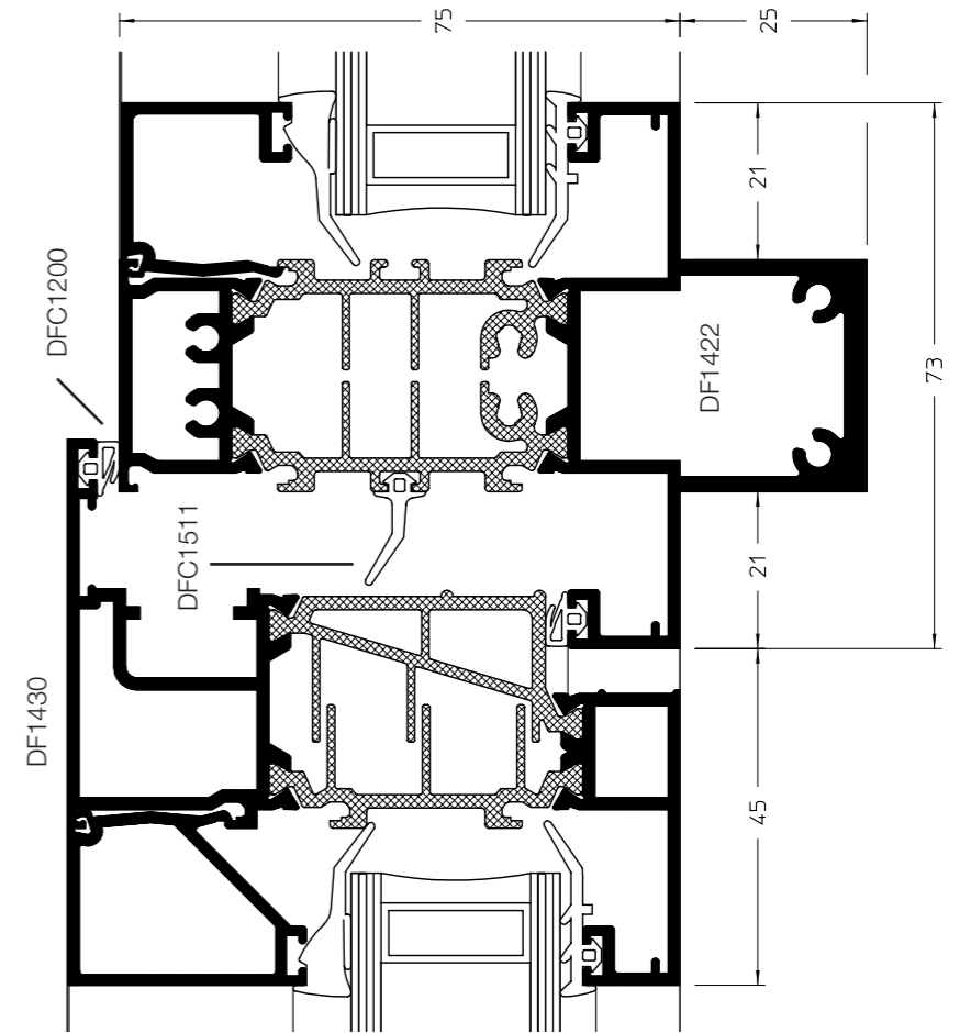
D Heavy Duty Mullion/Transom 73mm
